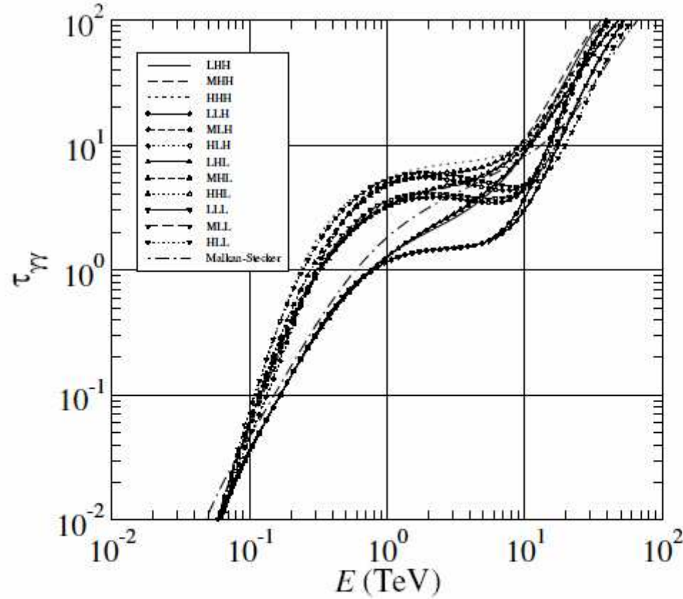
Fig. 1.— Optical depth calculated by the EBL models of Dwek & Krennrich (2005). The \gamma -ray energy in the observer's frame is denoted by E . The redshift of the \gamma -ray source is assumed to be 0.129. The optical depth calculated by Malkan-Stecker model is also shown for comparison ( dot-dashed ).
