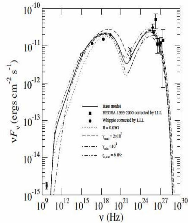
Fig. 5.— SED models calculated by different parameter values. Data from Whipple and HEGRA 1999-2000 are corrected by \exp(\tau_{\gamma\gamma}) with an EBL model, LLL. Base model denotes the SED shown in Fig. 2 by the dashed line.
